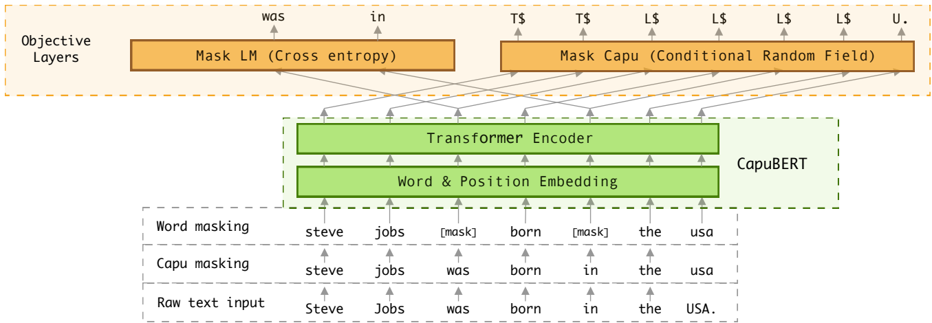
Fig. 1. Overview of the pre-training CapuBERT model. The raw text input ‘Steve Jobs was born in the USA.’ firstly goes through the capu masking process to remove capu information: ‘steve jobs was born in the usa’ and create capu labels: ‘T$ T$ L$ L$ L$ L$ U.’. Word masking process then randomly masks 15% words: ‘steve jobs [mask] born [mask] the usa’. Model is trained to detect masked words using Mask LM layer and predict capu labels using Mask Capu layer.
