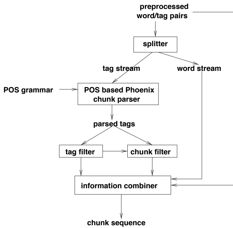
Figure 3.3: POS Chunk Parsing System
