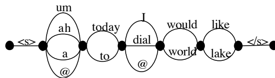
Fig.1 Confusion Network.
