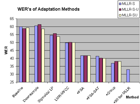
Figure 3: WER's of Adaptation Methods
