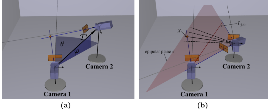
Fig. 2. Pairwise extrinsic calibration. (a) The angles \theta and \varphi corresponding to translation T' . (b) The solution space for lov_2 (red overlay) in Camera 1's reference frame, given an observation X and fixed translation and roll values for Camera 2. L_{\text{join}} is represented by the red line segment on the epipolar plane \pi .
