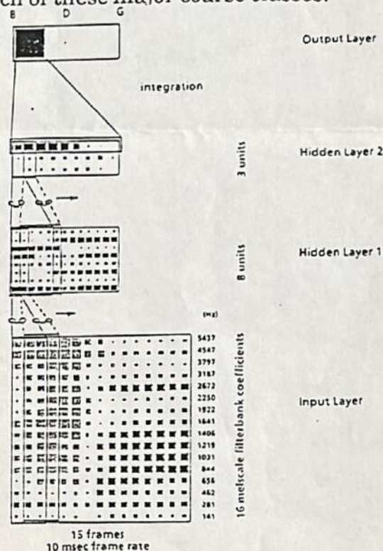
Fig. 1. The TDNN architecture (input: "BA")
