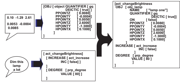
Figure 2: Multimodal Integration of Speech and Gestures
