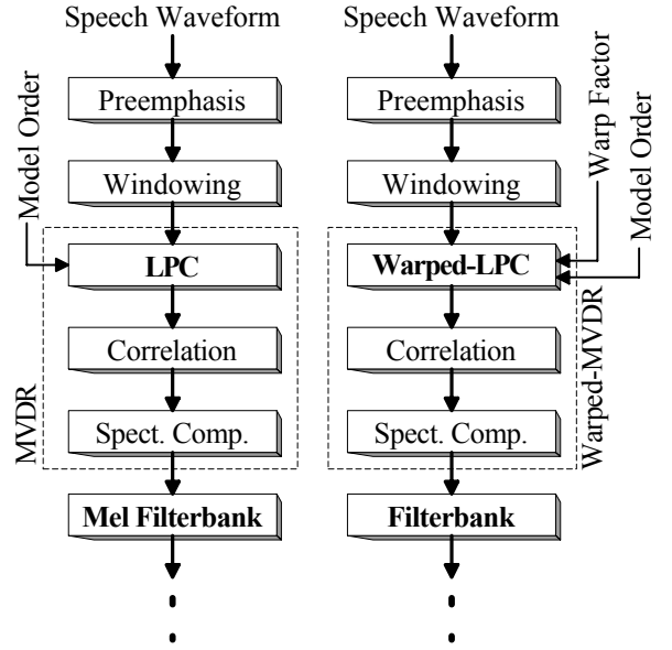
Figure 3: Extract of the MVDR (left) and the warped-MVDR (right) acoustic preprocessing used in our experiments.
