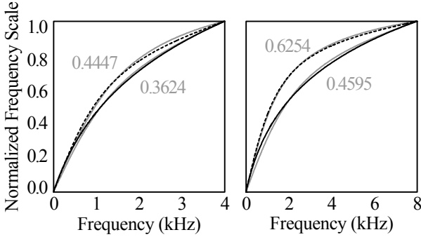
Figure 1: The approximations of Mel-frequency (black lines) and Bark-frequency (dotted black lines) by the bi-linear transformation (gray lines including the warping factor in gray digits) are demonstrated for 8 and 16 kHz sampling rates.
