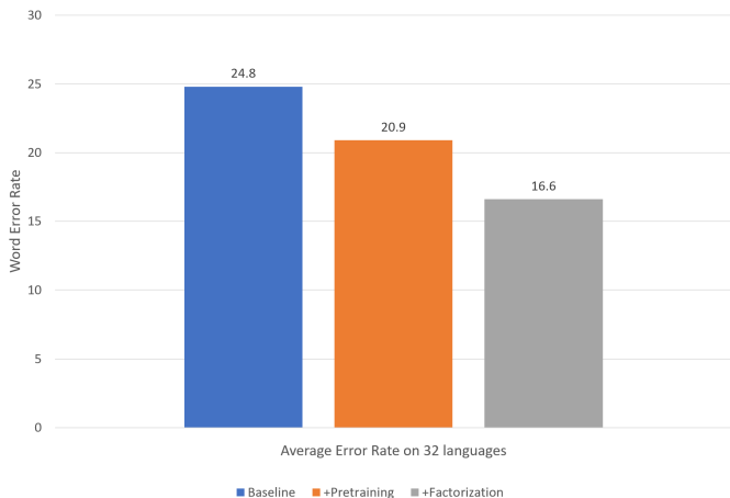
Figure 4.3: Summary of the results averaged on 32 languages.
