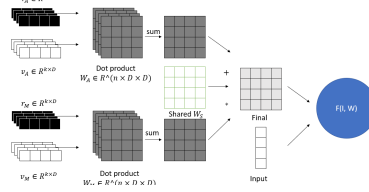
Figure 4.2: Weight factorization diagram. The per-language black and white parameters combine with the shared weight matrix to generate the specialized weight matrix W to transform input I .
