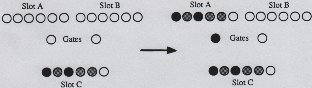
Figure 1: Gating Units
