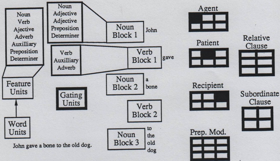
Figure 2: Network Structure
