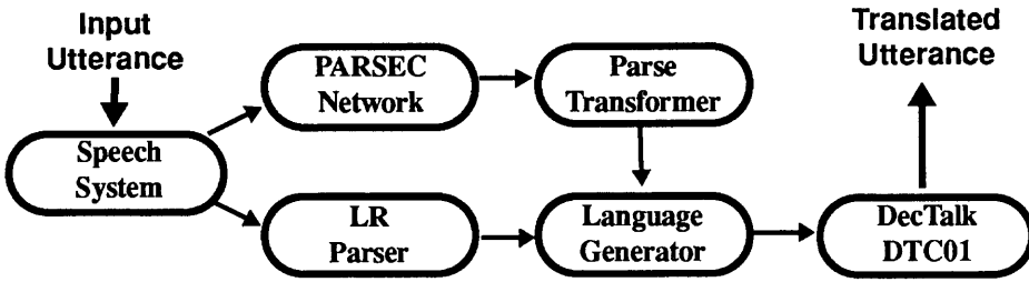
Figure 1: High-level JANUS architecture
