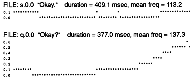
Figure 3: Smoothed pitch contours.
