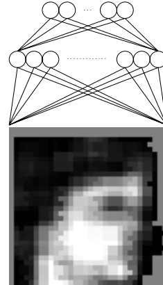
Figure 3: Network architecture
