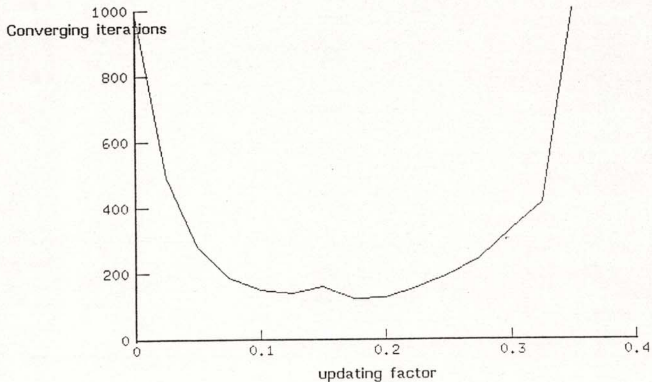
Figure 13: Number of converging Epochs vs. Step Size updating factor (838 task)
