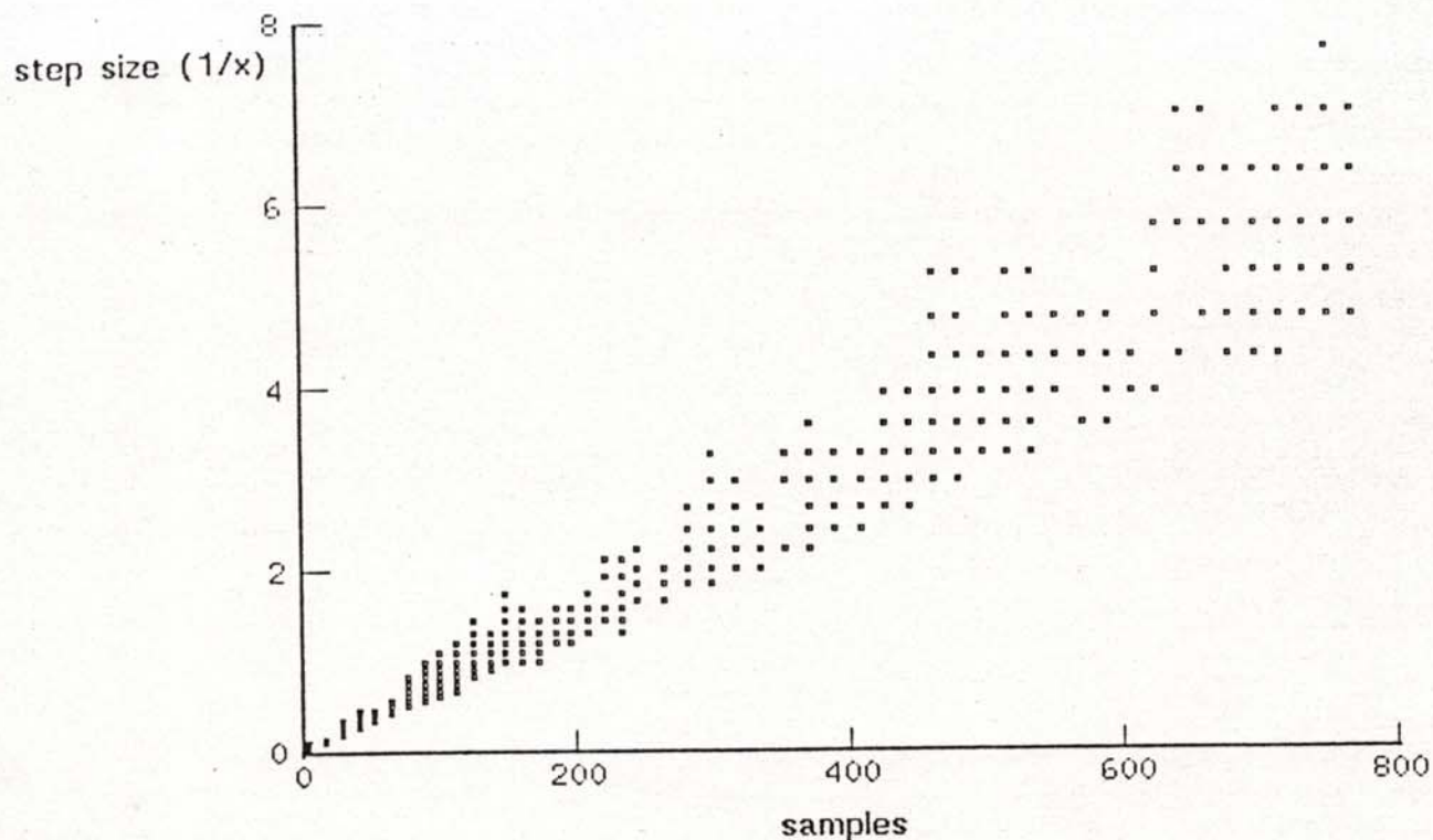
Figure 12: Optimal Step Size vs. Number of Training Samples (BDG task)
