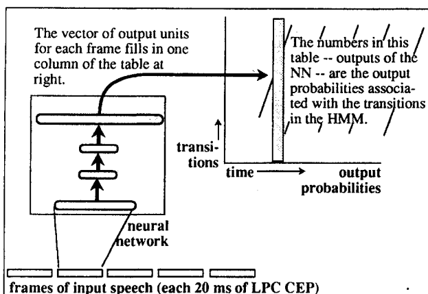
Figure 1a: NN Generation of Output Probabilities
