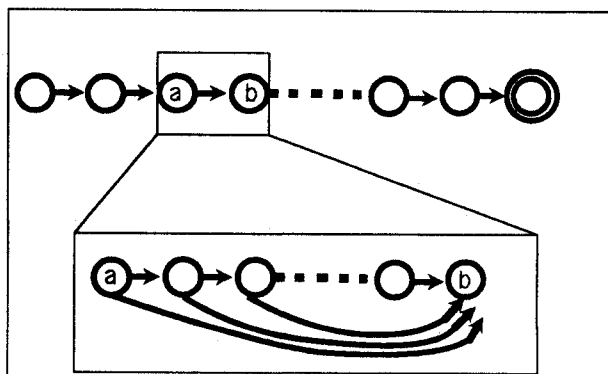
Figure 4a: Our Word Model
