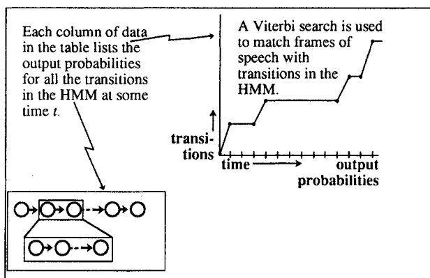
Figure 1b: HMM alignment of speech
