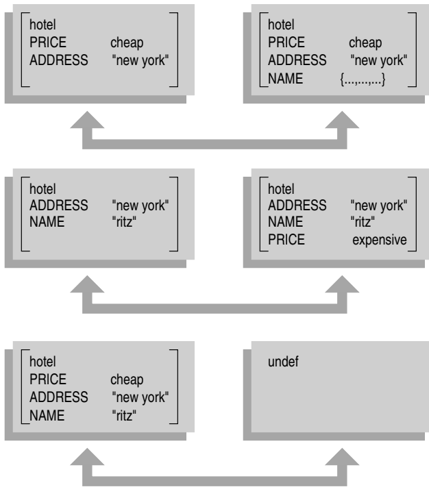
Figure 8: Different representation of descriptions and their referents. The first description refers ambiguously to a set of objects that is compactly represented in an underspecified feature structure. The second description refers uniquely to one object. The third description is overspecified; no object in the data base fits the description. The representations are depicted in a simplified fashion.
