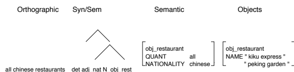
Figure 6: The four different levels of representation. At all times, the dialogue manager has access to all four levels and may pass any information on to other processing modules without being restricted by a static flow of information
