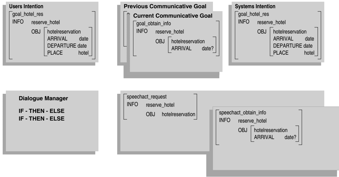
Figure 7: The overall architecture of the system. The users intention is to make a hotel reservation. The system opens a subdialogue in order to inquire the arrival date. The communicative goal of the user is temporarily replaced by the goal the generated by the system-initiated subdialogue. However, the intentions of user and system remain unchanged as the hotel reservation could not yet take place. Only the semantic layer of the four-layered blackboard is shown. The representations shown are simplifications of the representations actually used in the system.
