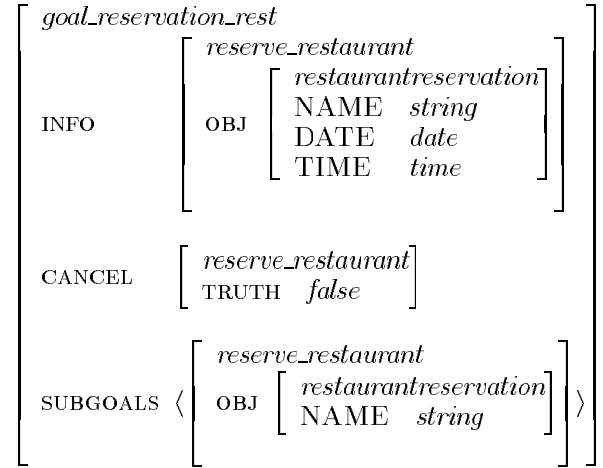
Figure 5: Strictly lower bounds of the information necessary to perform a restaurant reservation is represented in the value of the INFO feature. The CANCEL feature represents information that will remove the goal from the stack and thus represents an escape condition. The SUBGOALS feature returns a value of lower bounds on information that, if satisfied, trigger the execution of subgoals while not changing the stack of persistent goals.
