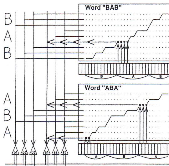
Figure 7. Training a Linked Predictive Neural Net
