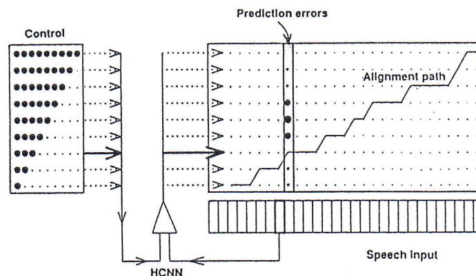
Figure 6. The Hidden Control Neural Network
