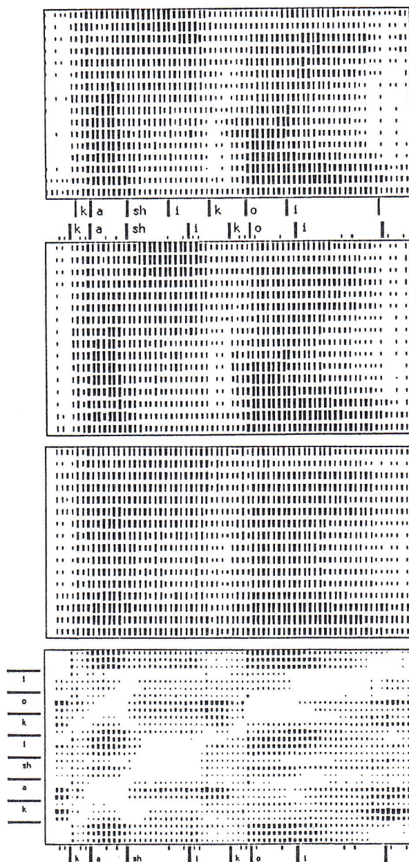
Figure 8. LPNN prediction for the word "kashikoi" (See text for explanation)
