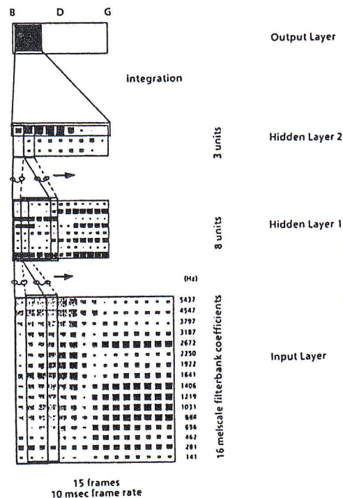
Figure 1. The TDNN architecture (/b,d,g/-task)
