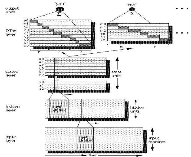
Figure 1. MS-TDNN architecture as used for handwriting recognition.
