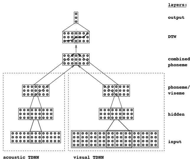
Figure 3. Basic recognition network architecture (integration at the phoneme/viseme level).
