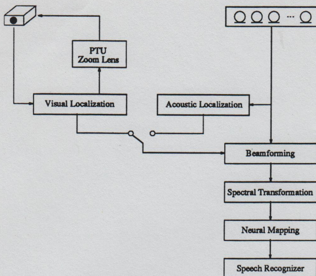
Figure 2. Acoustical and visually guided beamforming.
