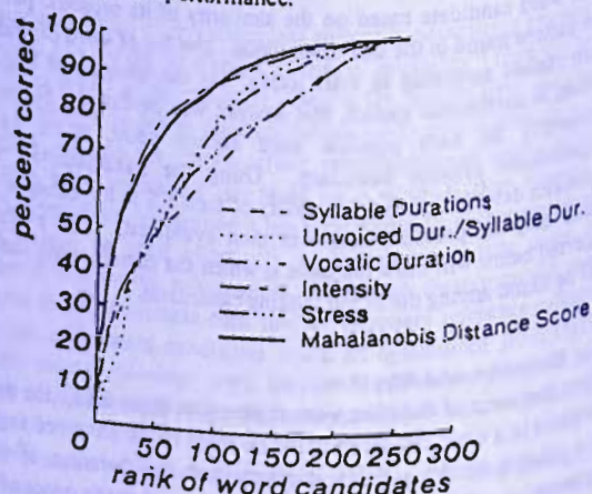
Figure 5. Combination of Prosodic Knowledge Sources
