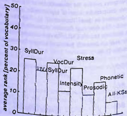
Figure 6. Comparison of Prosodic and Phonetic Knowledge Sources
