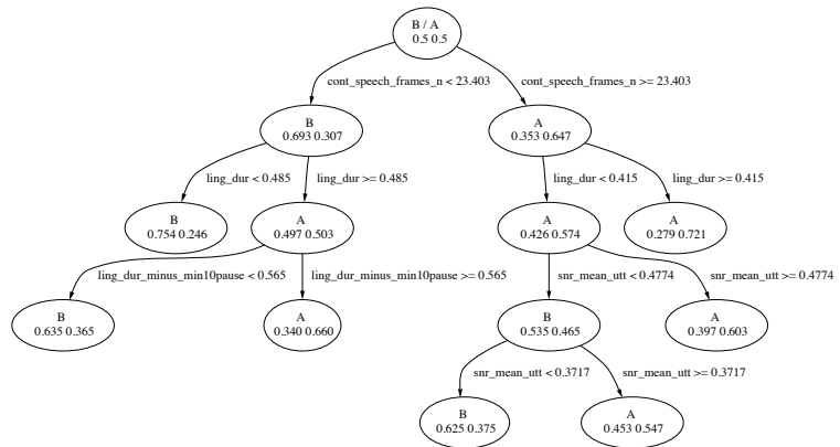
Figure 1: Decision tree for the classification of Backchannels (B) and Agreements (A). Each node is labeled with the majority class for that node, as well as the posterior probabilities of the two classes.
