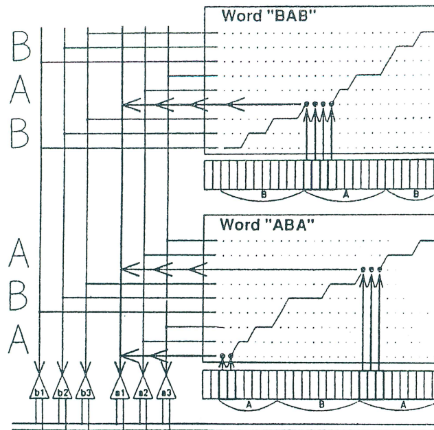
Figure 7. Training a Linked Predictive Neural Net
