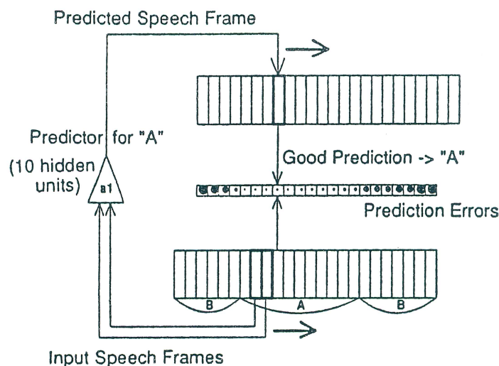
Figure 4. Modeling a phoneme by signal prediction
