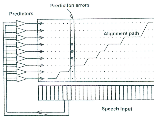
Figure 5. A Neural Prediction Model
