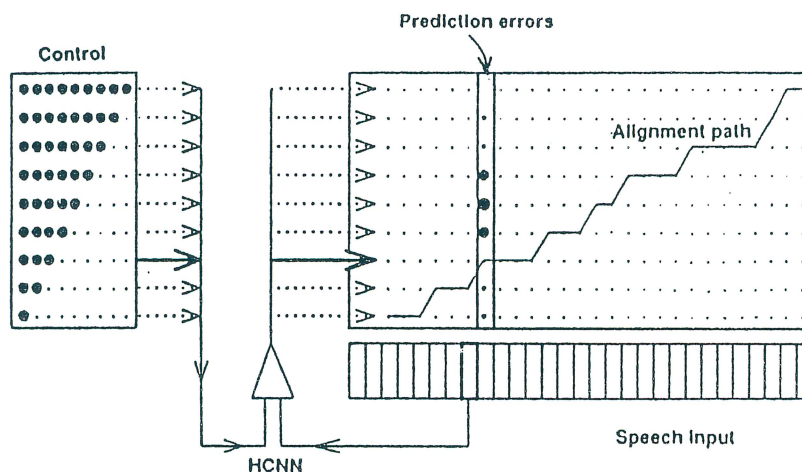
Figure 6. The Hidden Control Neural Network
