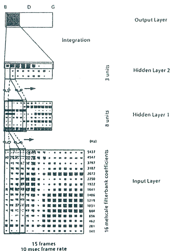
Figure 1. The TDNN architecture (/b,d,g/-task)
