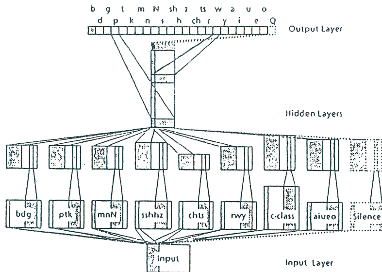
Figure 2. Modular TDNN used to spot all phonemes
